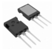
IXFX44N55Q IXYS MOSFET N-CH 550V 44A PLUS247
