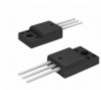
FFPF20UA60DN AMI Semiconductor / ON Semiconductor DIODE ARRAY GP 600V 10A TO220F
