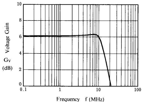
Voltage Gain vs. Frequency (Clamp Type Input) ( T_a = 25^\circ\text{C} , V^+ = 5V , 1V_{p-p} sinewave signal input)
