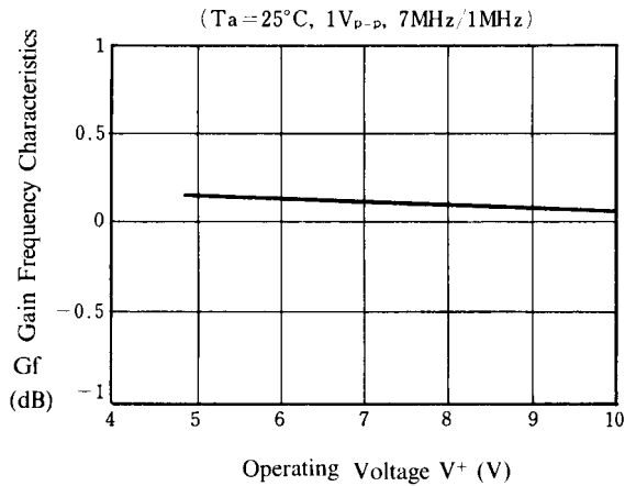
Gain Frequency Characteristics vs. Operating Voltage (Clamp Type Input) ( T_a = 25^\circ\text{C} , 1V_{p-p} , 7MHz/1MHz)
