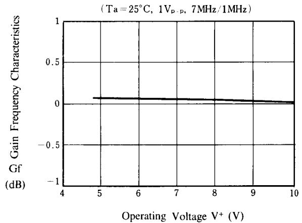
Gain Frequency Characteristics vs. Operating Voltage (Bias Type Input) ( T_a = 25^\circ\text{C} , 1V_{p-p} , 7MHz/1MHz)
