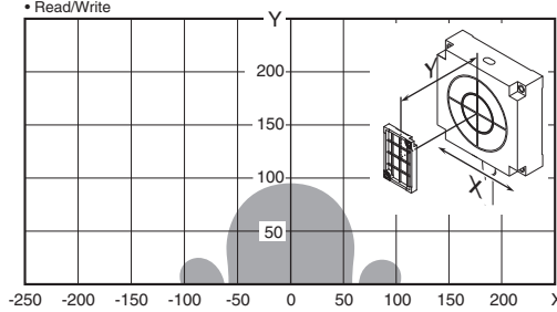
V680-HS65 (mounted on metallic material) & V680S-D8KF68M (Metal on back: Steel (Tag direction: Vertical))
