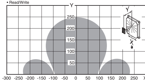
V680-HS63 (mounted on non-metallic material) & V680S-D8KF68M (Metal on back: Steel (Tag direction: Vertical))
