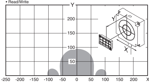
V680-HS65 (mounted on metallic material) & V680S-D8KF68M (Metal on back: Steel (Tag direction: Horizontal))
