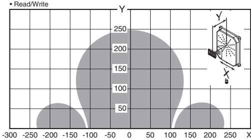
V680-HS63 (mounted on non-metallic material) & V680S-D8KF68M (Metal on back: Steel (Tag direction: Horizontal))
