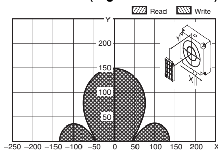
V680-HS63 (with Metal on Back Surface) & V680S-D2KF68M (Metal on back: Steel) (Tag direction: Horizontal) V680S-D2KF68M (Metal on back: Steel) (Tag direction: Vertical)
